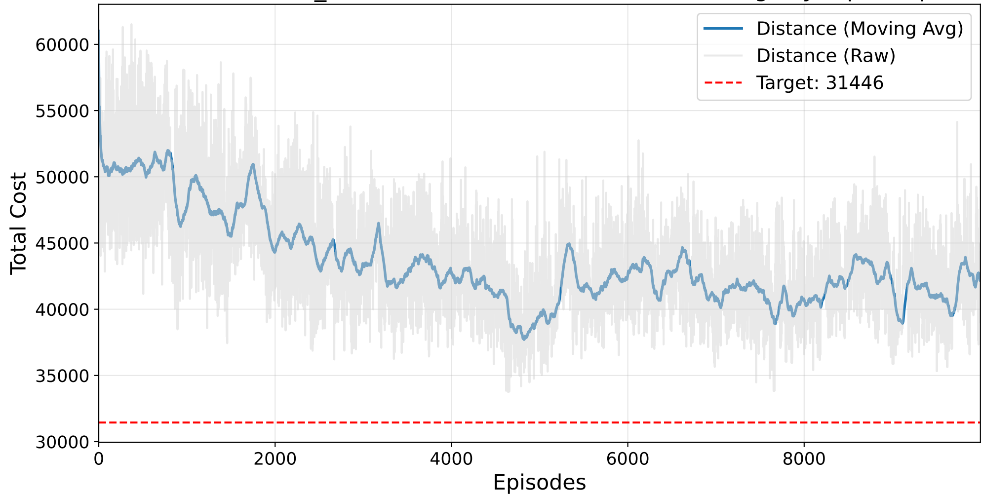
Final RANDOM_SEARCH Masked AutoRL-SOP Training - ry48p.4.sop
